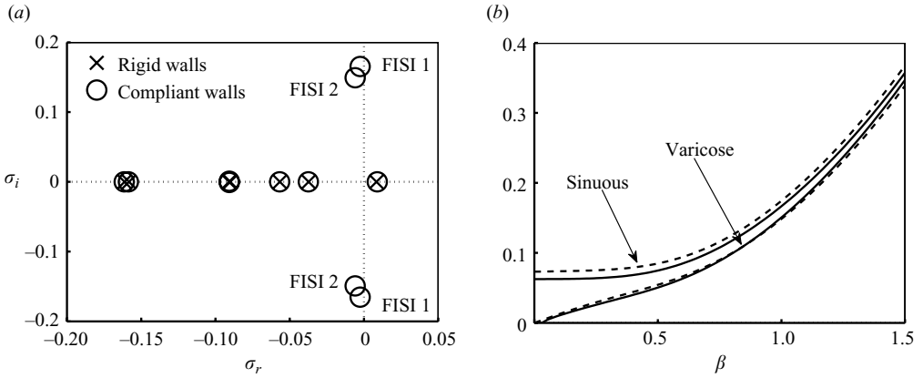
FIGURE 3. (a) Comparison of the axisymmetric eigenvalue spectrum for the rigid-wall and compliant-wall cases for \beta = 1 and Re = 250 . The hydroelastic modes are labelled FIS1. (b) Frequency of the sinuous-like and varicose-like axisymmetric FIS1 modes (solid lines) compared to the results obtained using the added mass model (dashed lines) for Re = 250 . The wall parameters are B = 4000 , K = B/4 and d = 0 .
