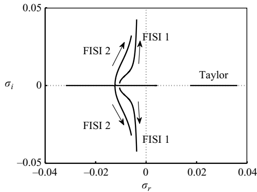
FIGURE 4. Evolution of the main axisymmetric eigenvalues with the spanwise wavenumber ( 0.2 \leq \beta \leq 2 ). The parameters are Re = 250 , B = 400 , K = B/16 and d = 0 . Arrows denote increasing \beta .
